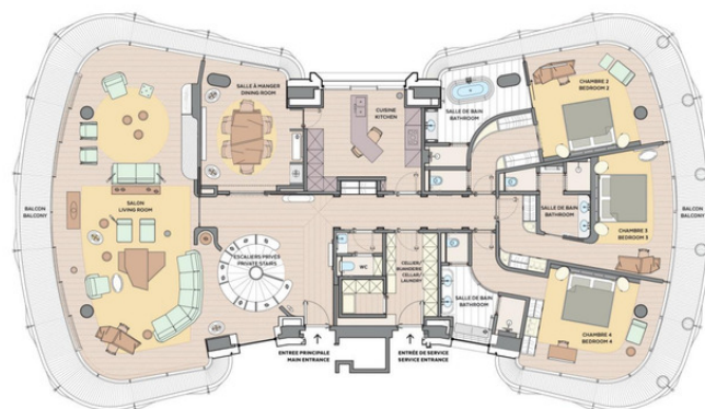
Main floor:
